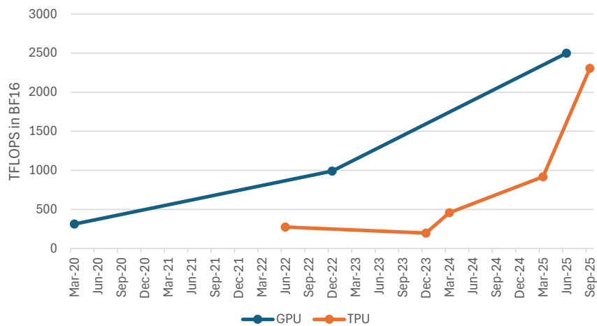
Figure 6: On a TFLOPS basis, GOOGL has made significant progress with TPU7x (Ironwood)
