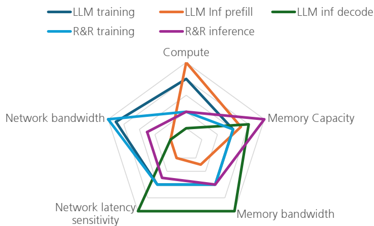
Figure 5: Varying requirements for different workloads
